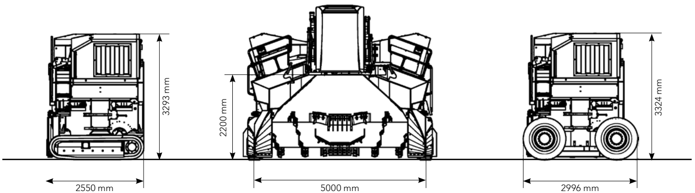
Track transport dimensions
